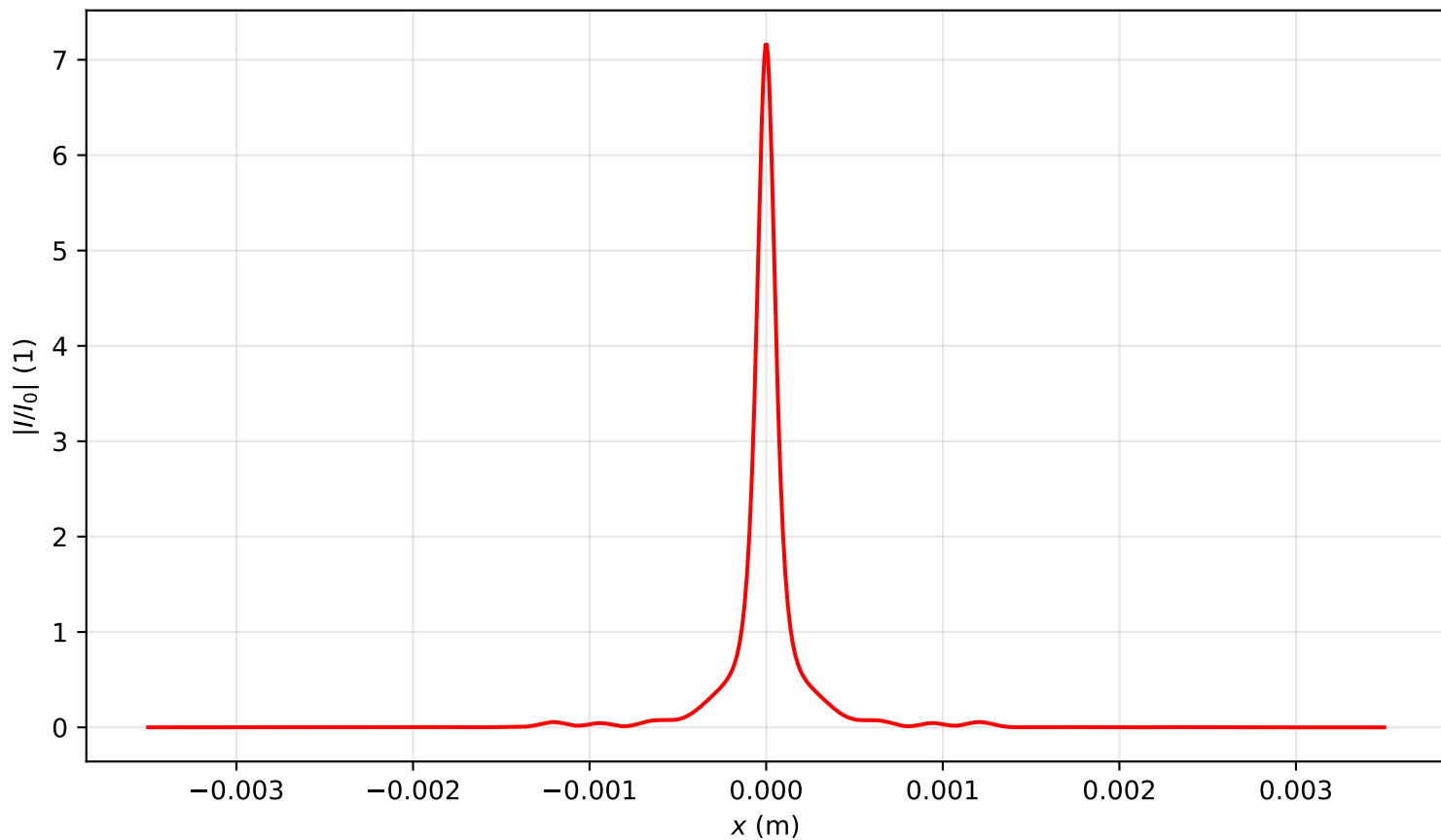
Intensity profile I(x, y = 0, z = 1.433)/I_0 , \text{Pin}=5.5\text{Pcr} , artificial time
